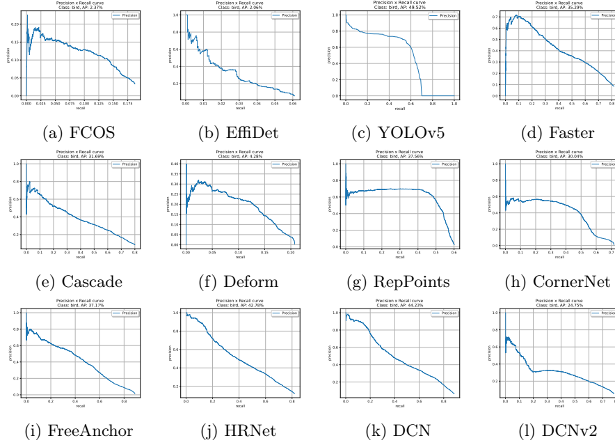
Fig. 8: Precision-Recall curves of different detectors in VOC[6] style.
